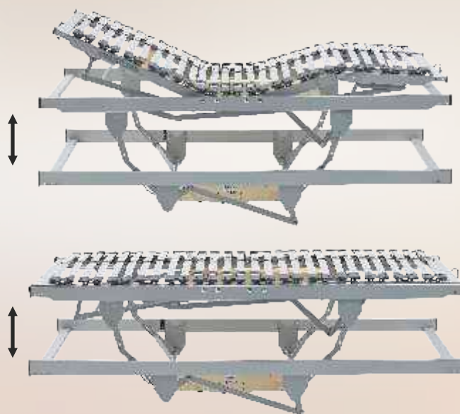
Carers' Hi-Low Mechanism (profiled, top and flat bottom)
